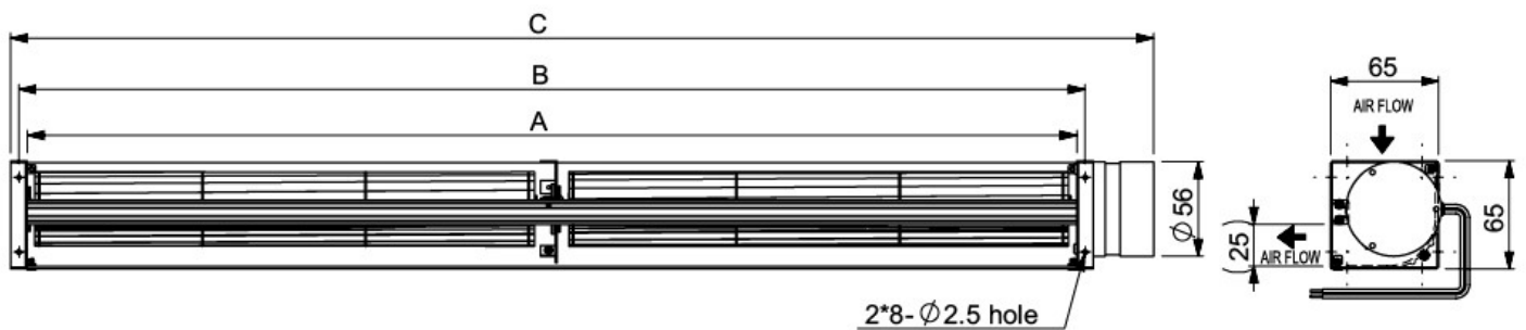
(Double Blower)
